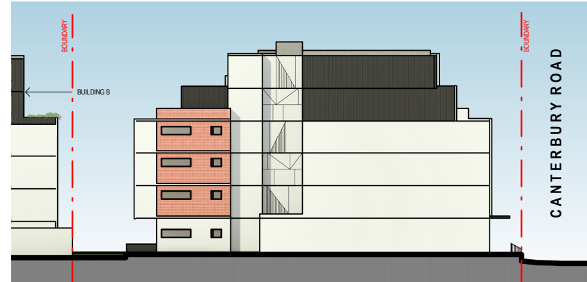
2 EAST ELEVATION - BUILDING A
