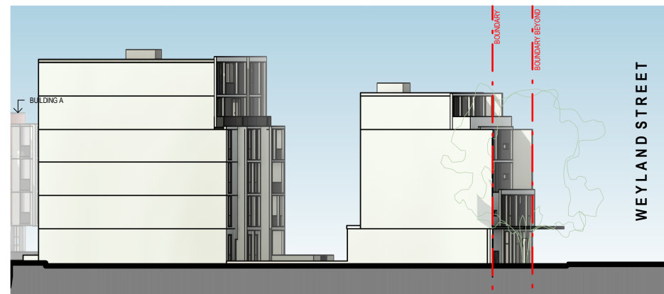
2 WEST ELEVATION - BUILDING B & C
